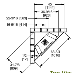
Top View Corner Installation
